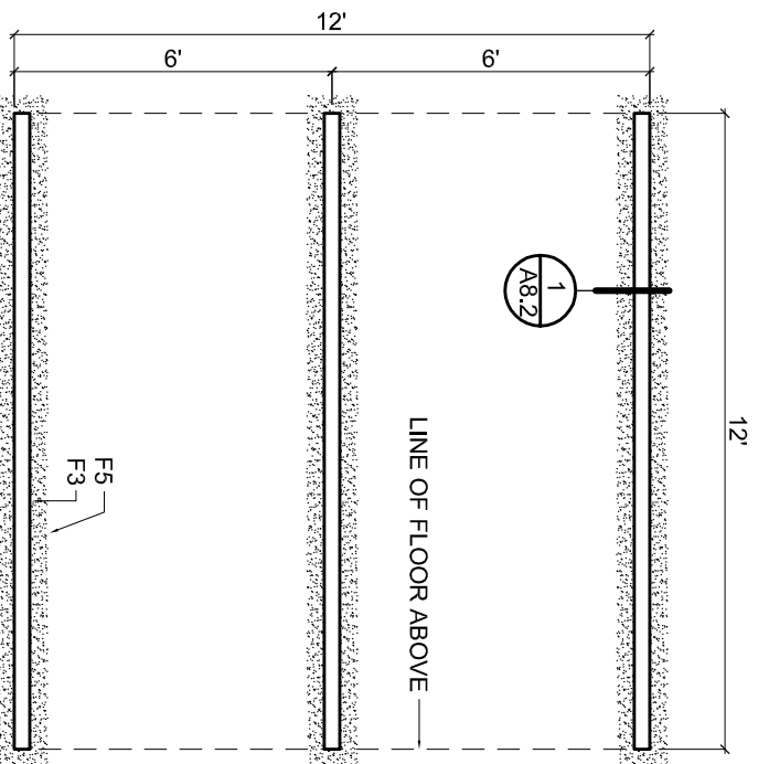
FOUNDATION RAIL FRAMING PLAN
